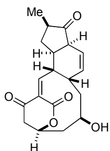
(+)-macquarimicin A (1) (revised structure)
